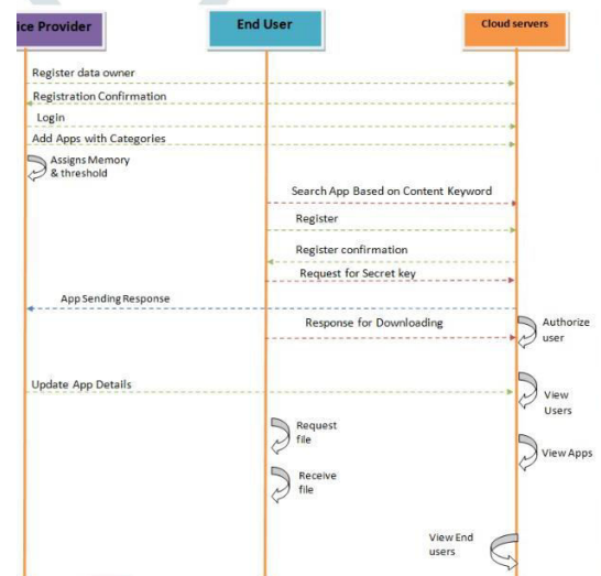
Fig 3.3.2: Sequence Diagram
